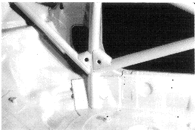
PHOTO N° 7 LATERAL BAR TO FLOOR
