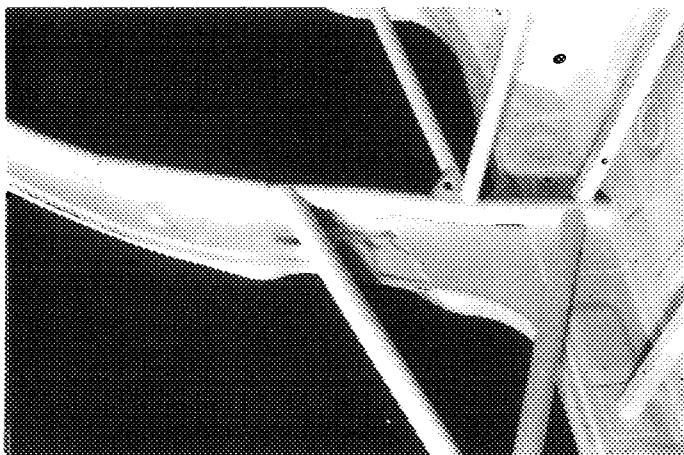
PHOTO N° 11 MAIN ROLLBAR TO B-PILLAR
