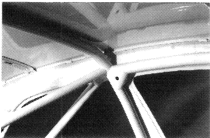
PHOTO N° 12 MAIN/LATERAL/DIAGONAL BAR JOINT
